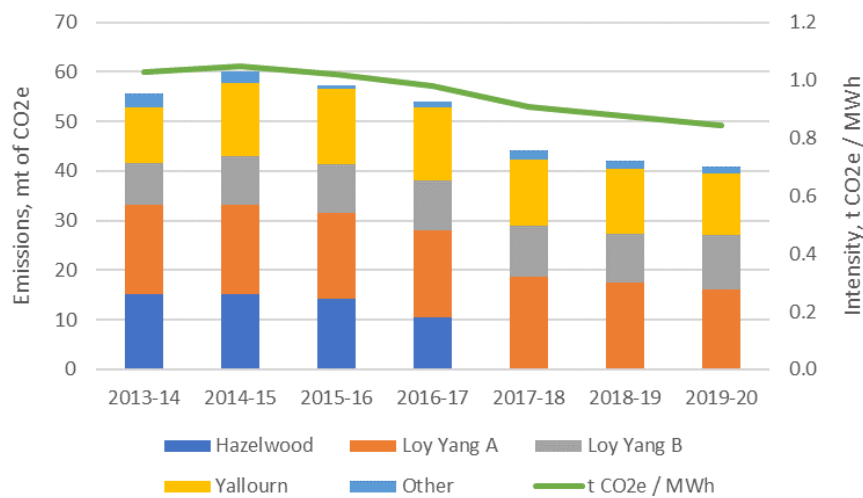
Figure 3: Emissions and emissions intensity of Victorian electricity generation, 2013-14 to 2019-20
