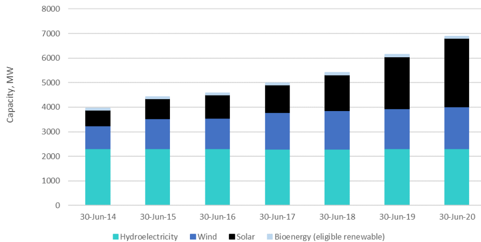
Figure 2: Victorian renewable electricity generation capacity, 2014 to 2020
